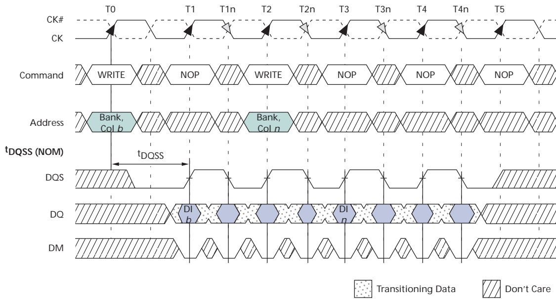
Figure 40: Consecutive WRITE-to-WRITE
